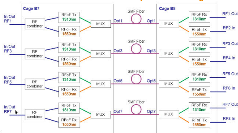
Bidirectional Multi-channel 4 RFoF sub-system block diagrams
