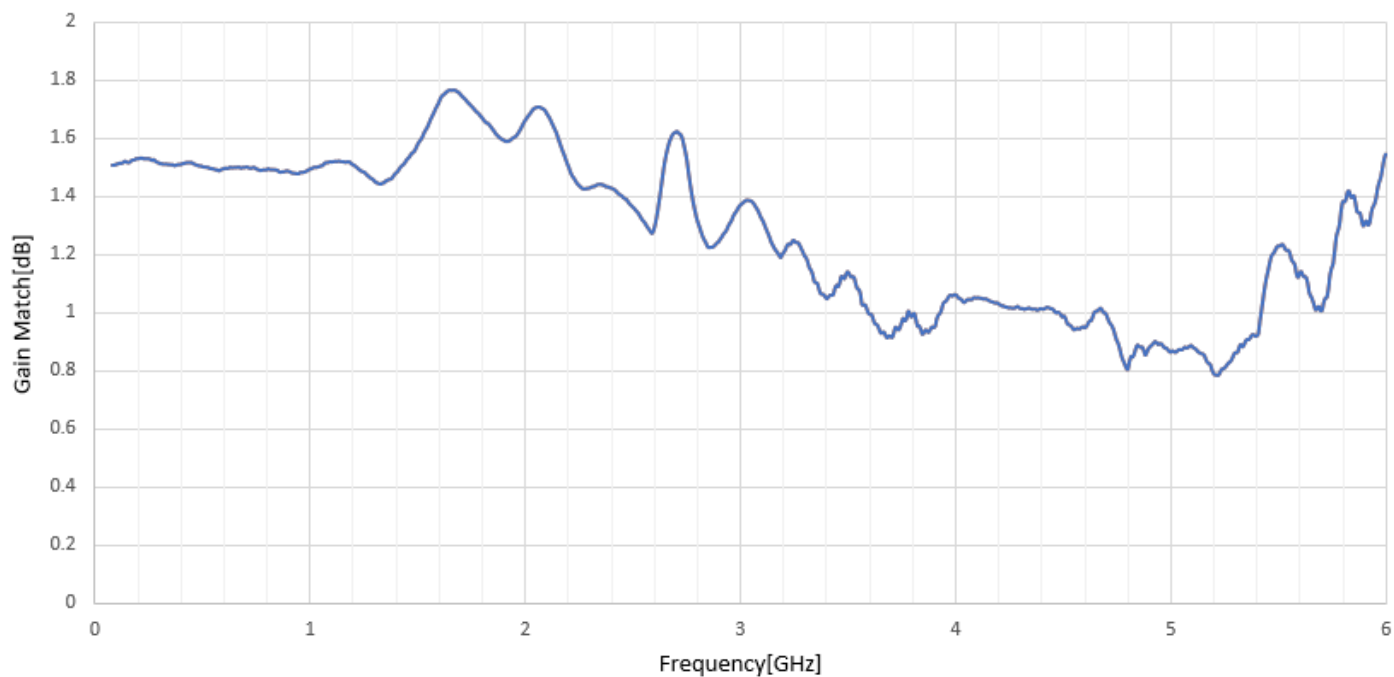
Overall Gain Deviation (Max - Min) in 100MHz to 6GHz Spec: \pm 2.5\text{dB}
